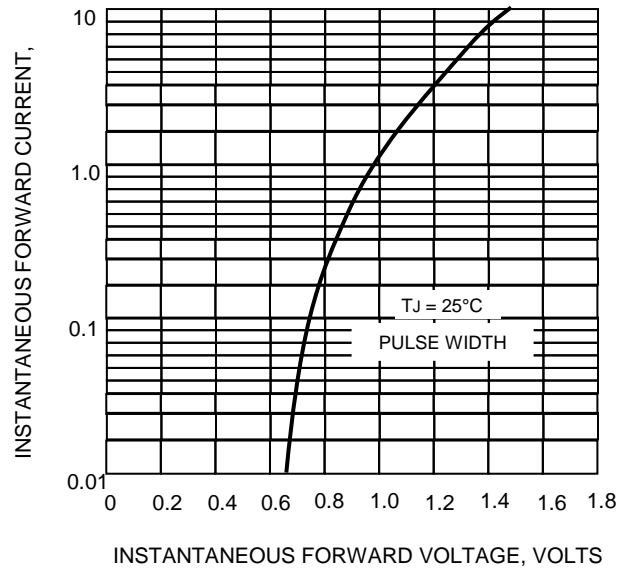
FIG.4-TYPICAL FORWARD CHARACTERISTICS
